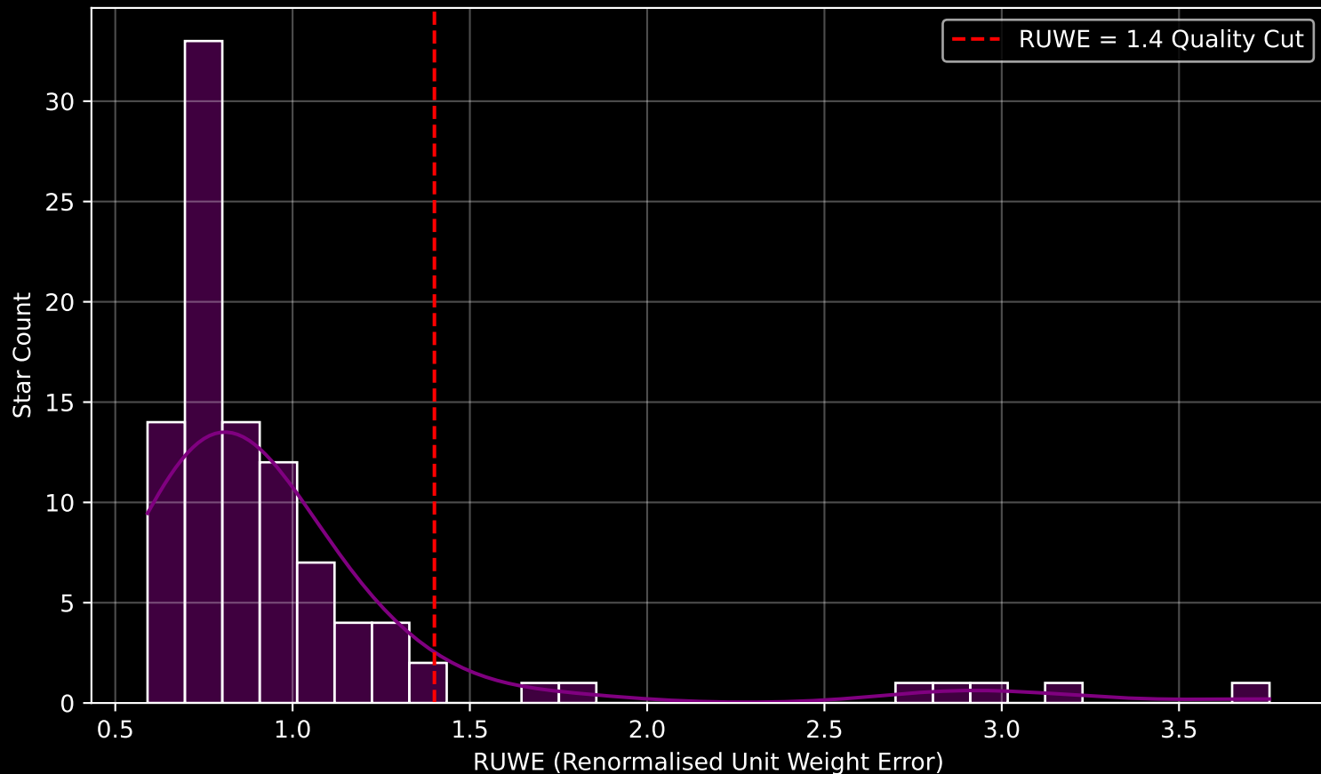
GAPOGEE DR17 Field [281-33-O_TESS] RUWE Distribution (n= 97)
