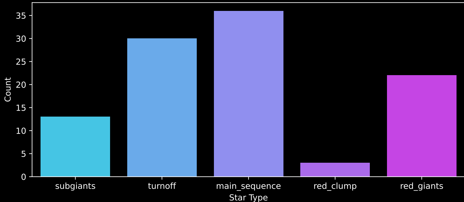
APOGEE DR17 Field: [281-33-O_TESS] Count plot of Star Type
